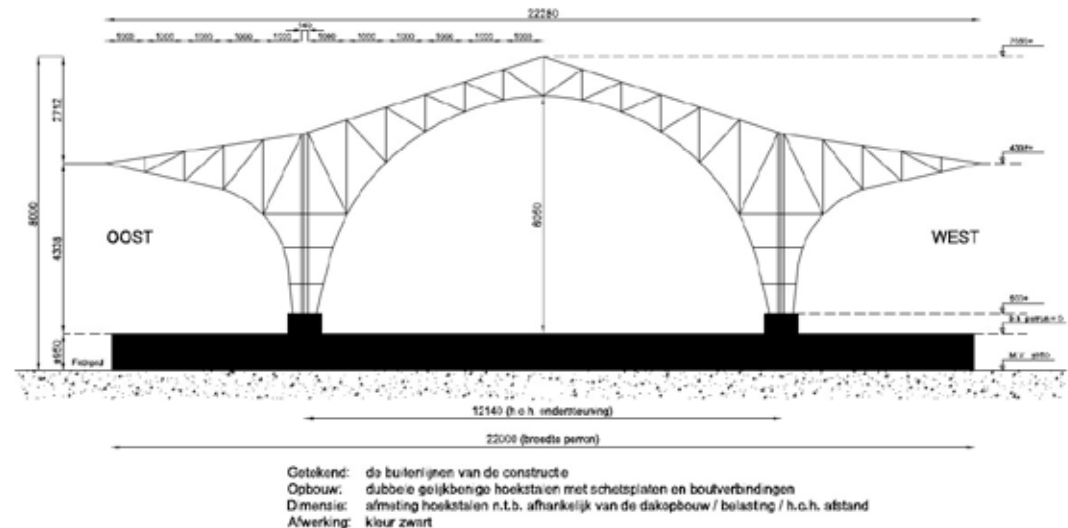
SCHEMA SPANT PERRON GRENS BAARLE-NASSAU / RAVELS
